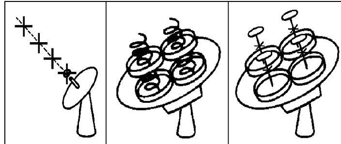
Figure 5.11 Four-Element Arrays by Ilcev 2013
