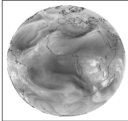
Figure 6. 18 Meteosat-1 Water Vapor Image by SSEC 2006
