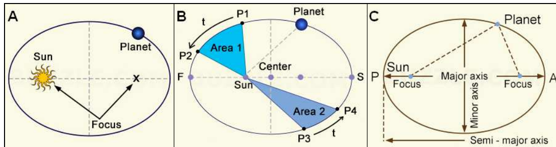
Figure 3. 1. Kepler's Laws of Satellite Motion by Ilceev 2011
